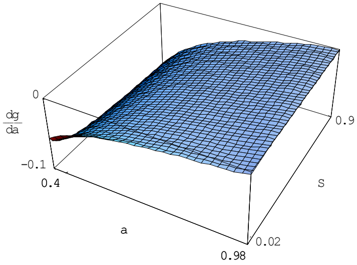
FIGURE 2b: \frac{dg}{da}
