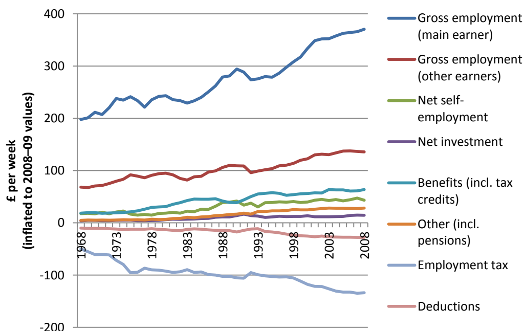
Figure 25. Average net equivalised household income by source
