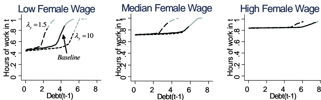
Figure 9: Labor Supply for Home-Owners by Debt varying \lambda_y
